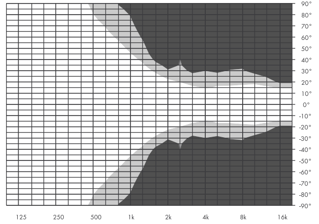
ALi60 vertical isobars
