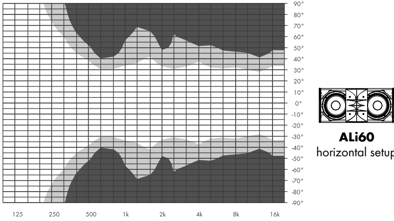
ALi60 horizontal isobars
