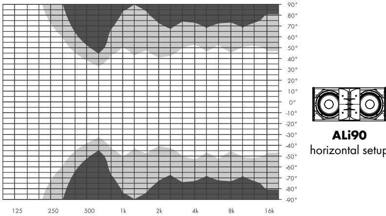
ALi90 horizontal isobars
