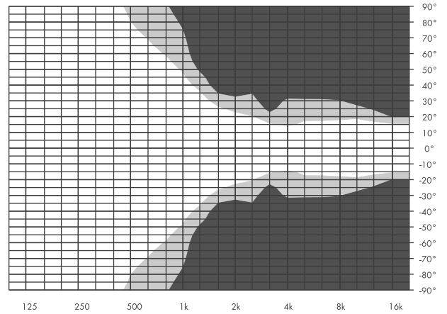
ALi90 vertical isobars
